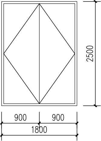
PM1825 1:50
