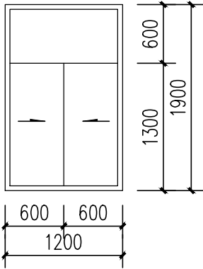
TC1219 1:50
