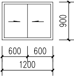
TC1209 1:50
