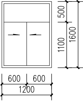
TC1216 1:50
