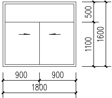
TC1816 1:50
